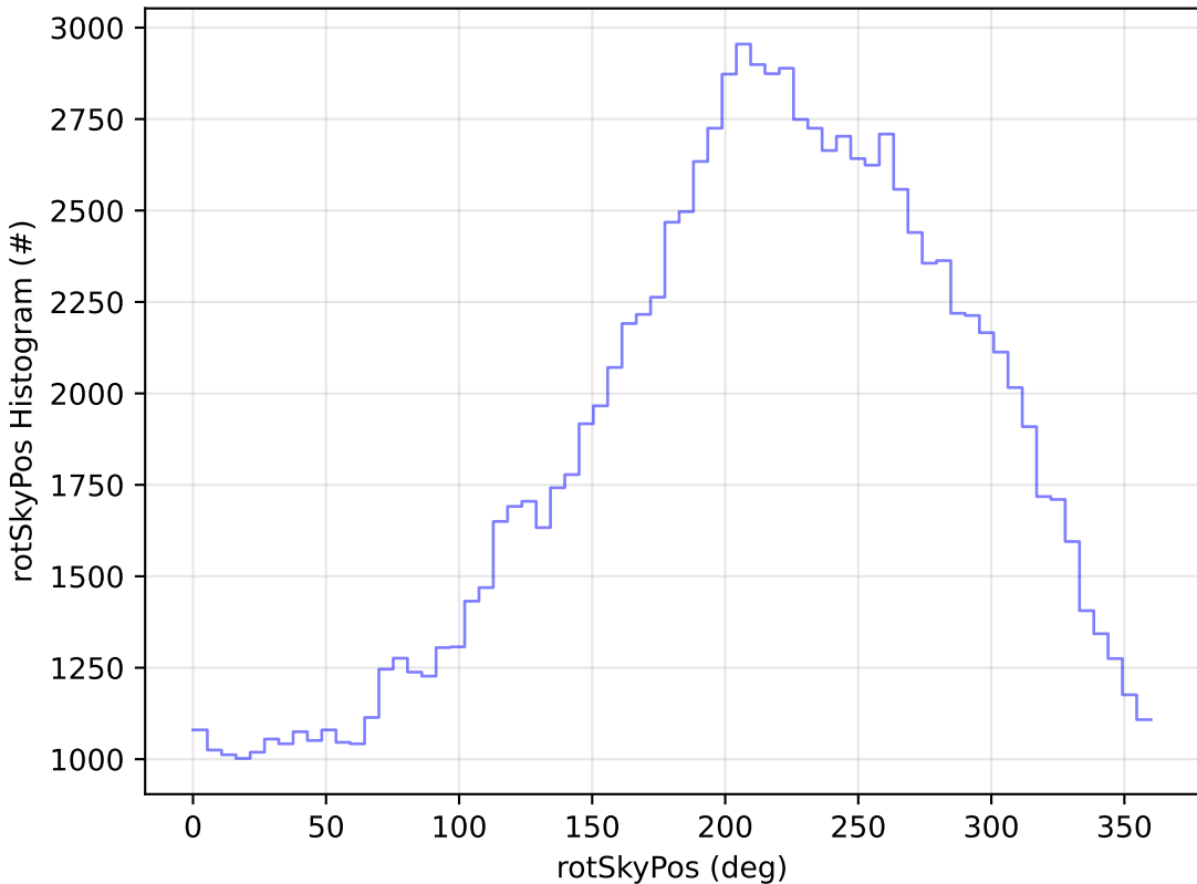
ddf_acor_sf10_lsf40_lsr20_v3.4_10yrs All sky u band: rotSkyPos Histogram
