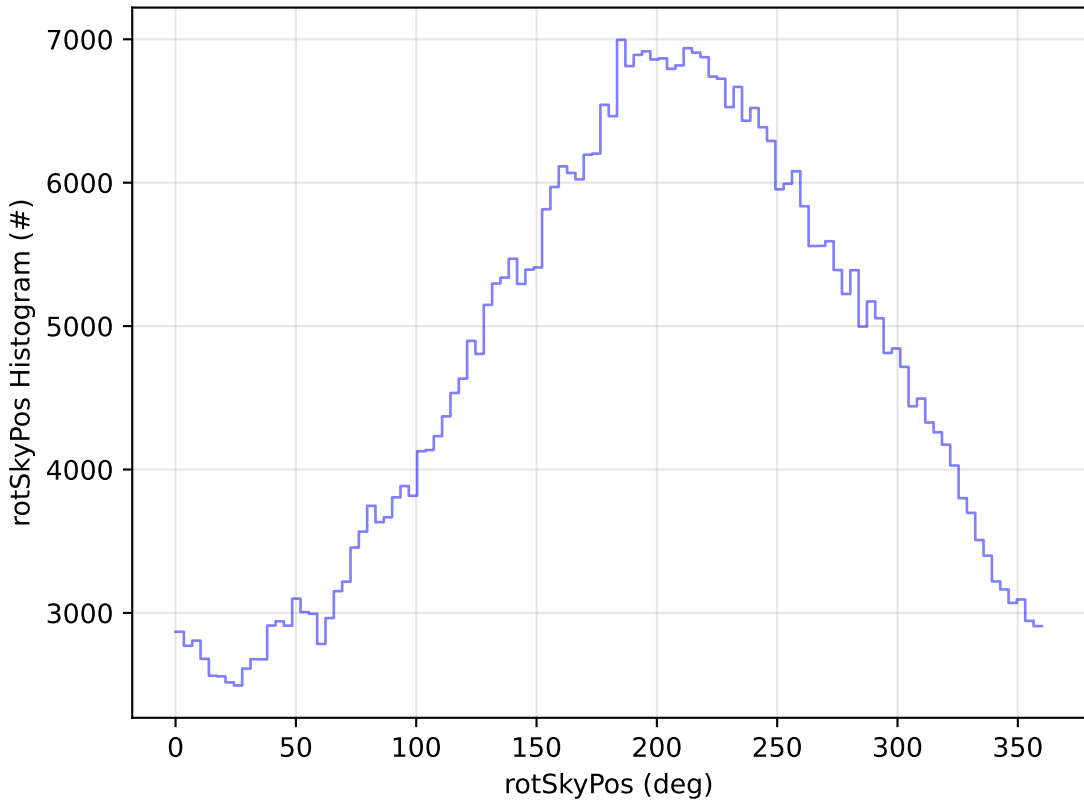
ddf_acor_sf10_ls40_lsr20_v3.4_10yrs All sky r band: rotSkyPos Histogram
