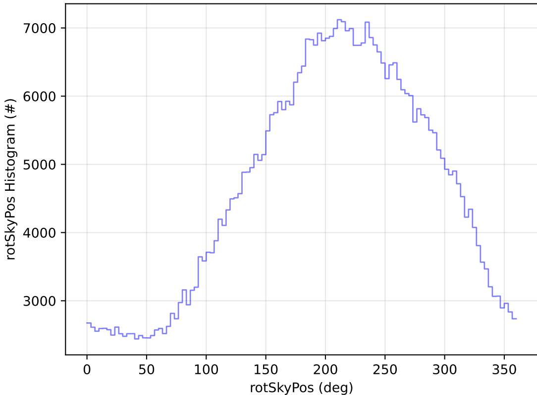
ddf_acor_sf10_lsf40_lsr20_v3.4_10yrs All sky i band: rotSkyPos Histogram
