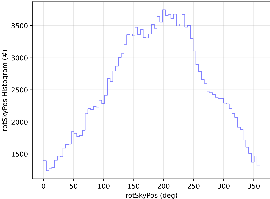
ddf_acor_sf10_lsf40_lsr20_v3.4_10yrs All sky g band: rotSkyPos Histogram
