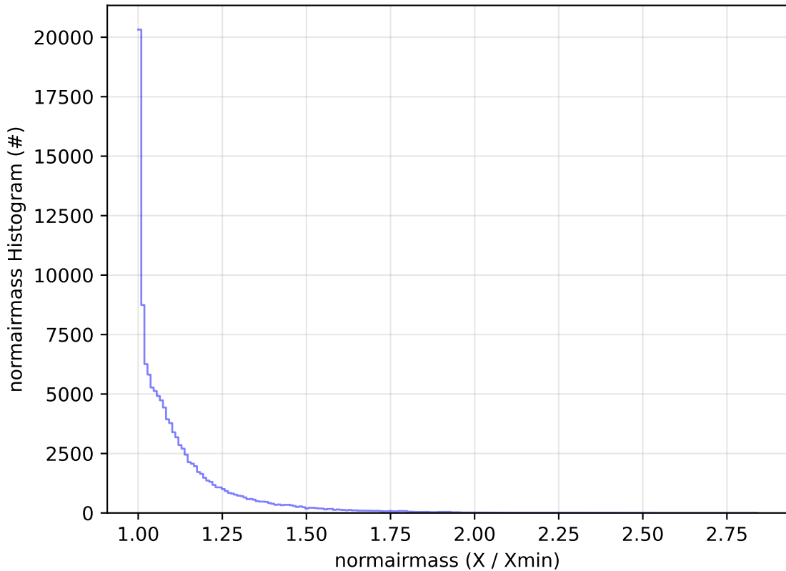
ddf_acor_sf10_lsf40_lsr20_v3.4_10yrs WFD u band: normairmass Histogram
