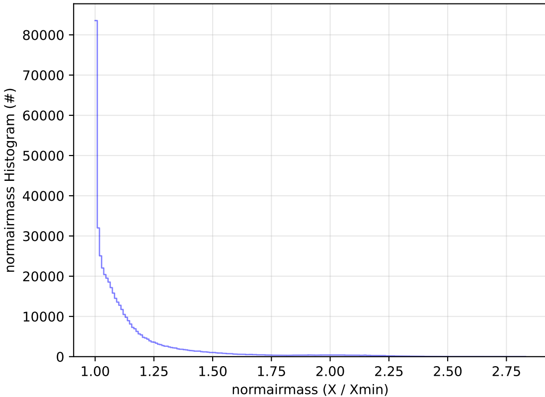
ddf_acor_sf10_lsf40_lsr20_v3.4_10yrs WFD r band: normairmass Histogram
