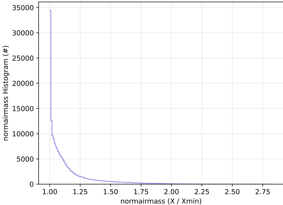
ddf_acor_sf10_lsf40_lsr20_v3.4_10yrs WFD g band: normairmass Histogram
