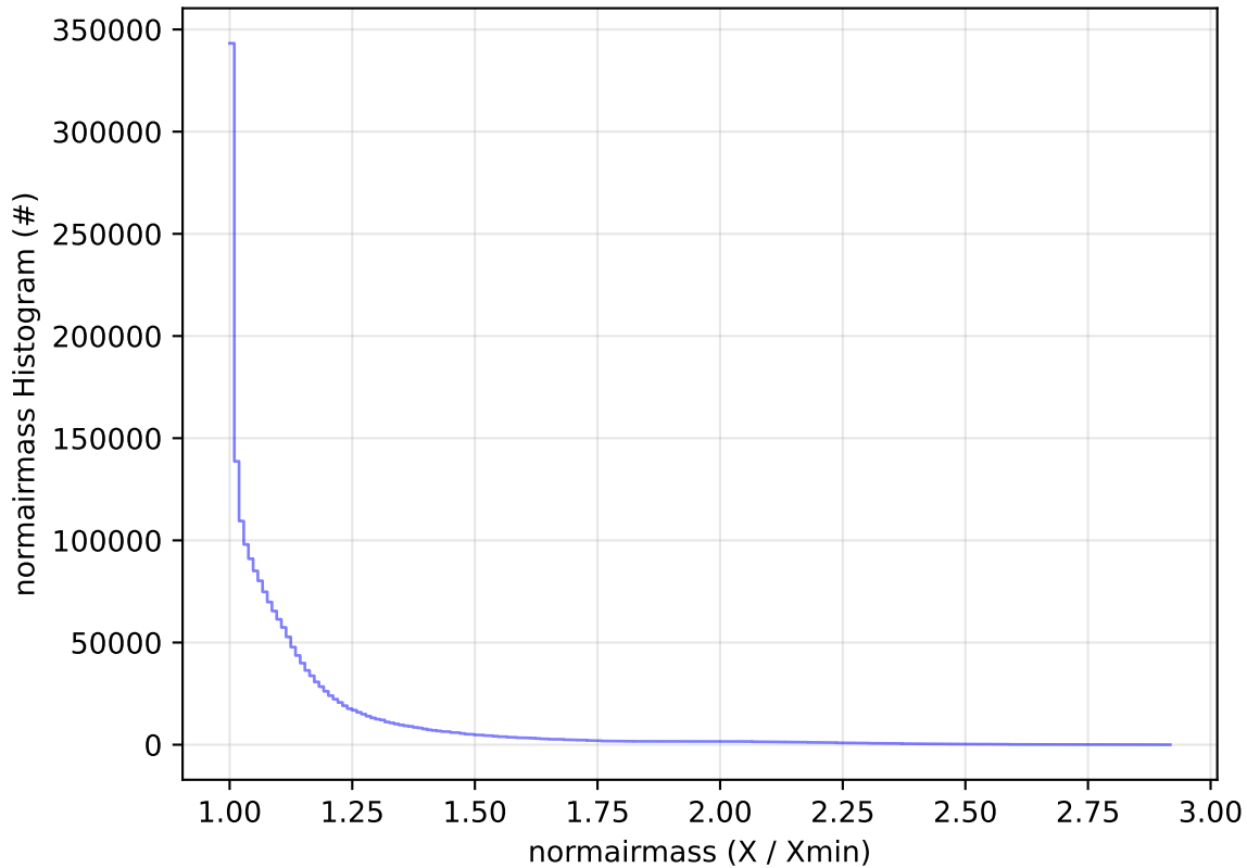
ddf_acor_sf10_lsf40_lsr20_v3.4_10yrs WFD all bands: normairmass Histogram
