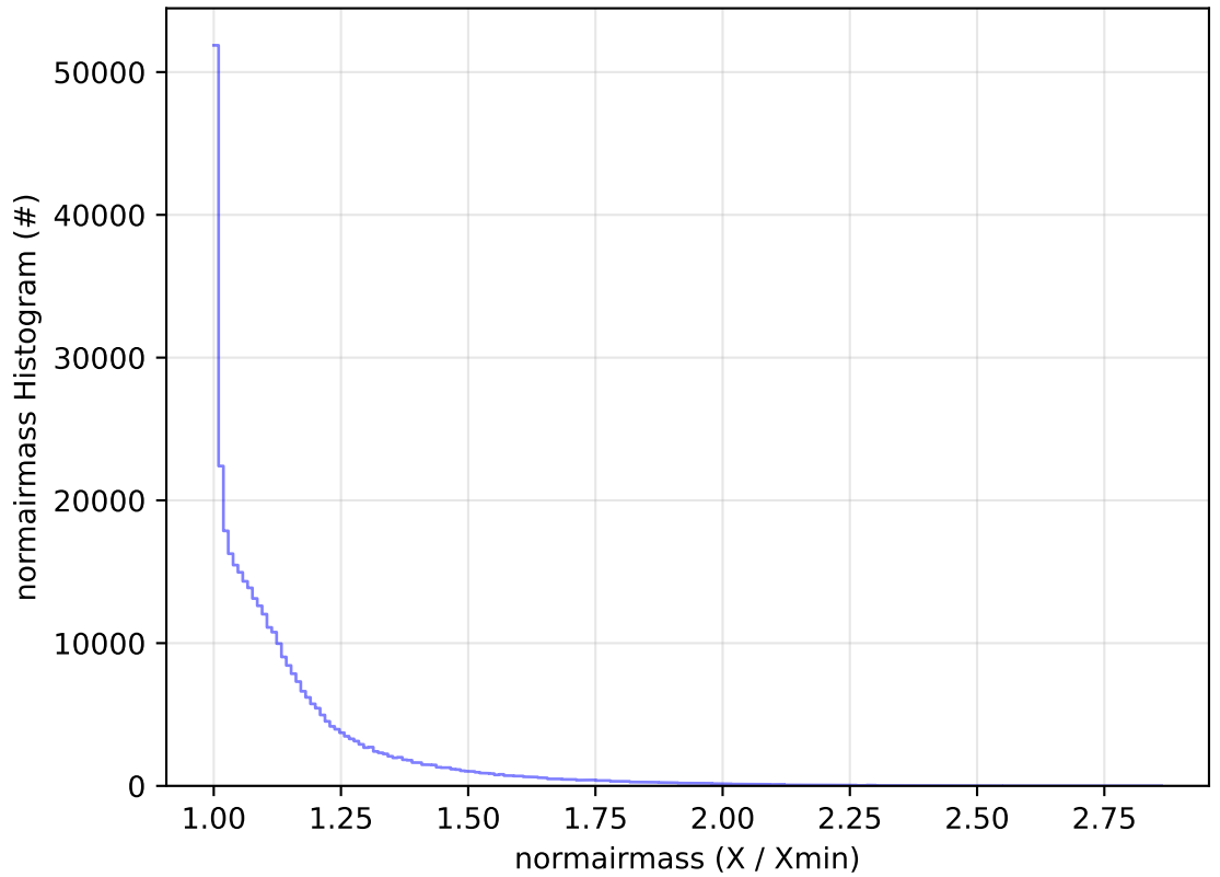
ddf_acor_sf10_lsf40_lsr20_v3.4_10yrs All sky y band: normairmass Histogram
