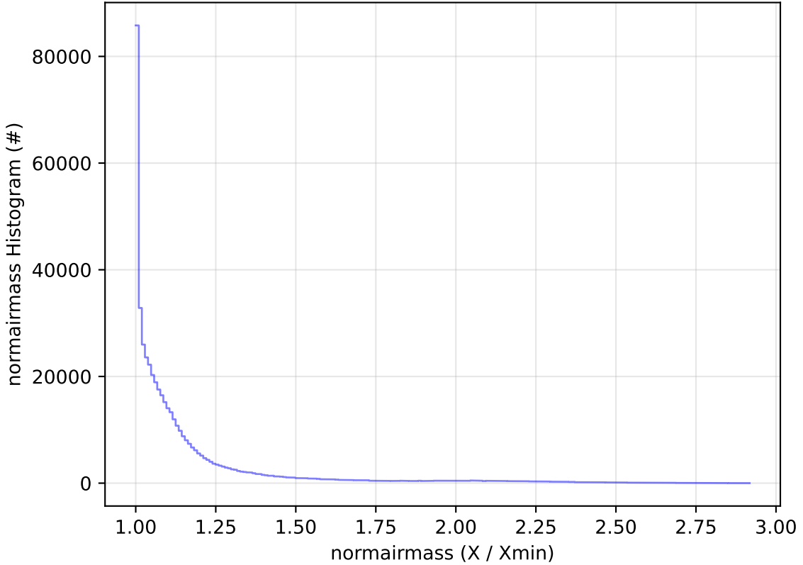
ddf_acor_sf10_lsf40_lsr20_v3.4_10yrs All sky i band: normairmass Histogram
