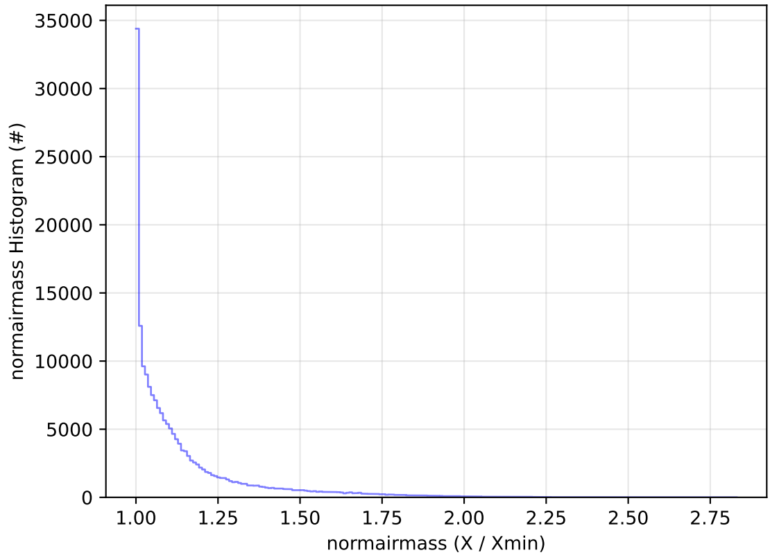
ddf_acor_sf10_lsf40_lsr20_v3.4_10yrs All sky g band: normairmass Histogram
