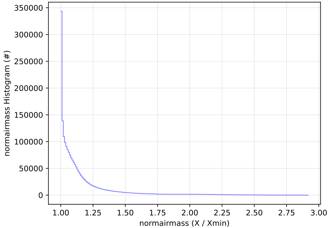
ddf_acor_sf10_lsf40_lsr20_v3.4_10yrs All sky all bands: normairmass Histogram
