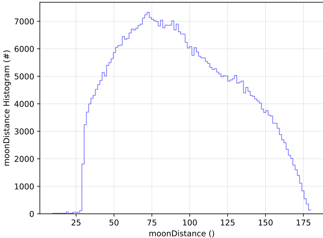
ddf_acor_sf10_lsf40_lsr20_v3.4_10yrs WFD i band: moonDistance Histogram
