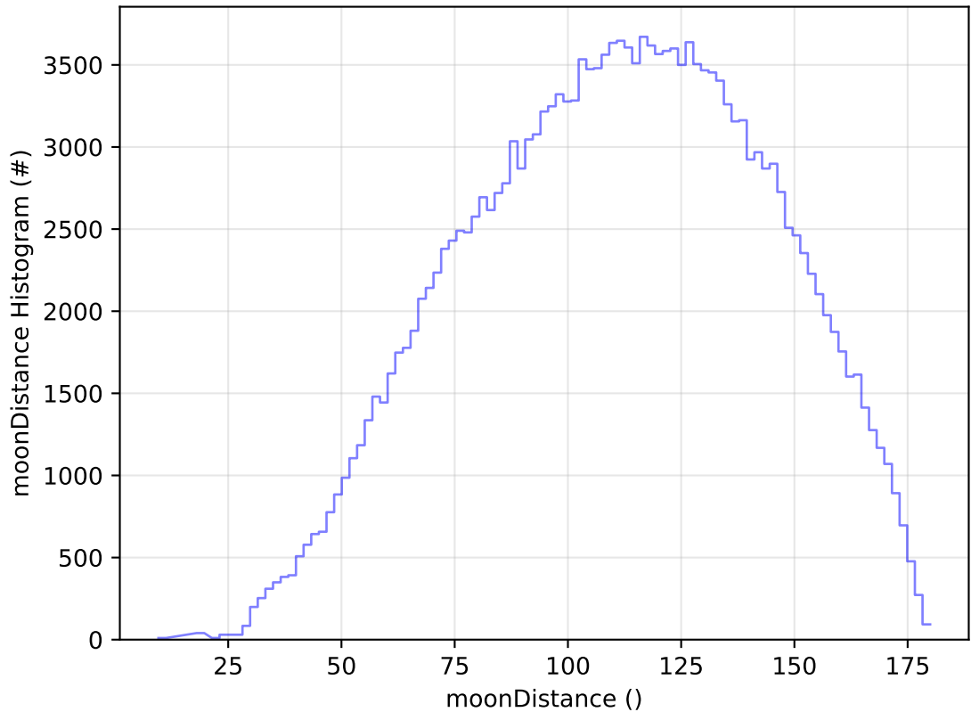
ddf_acor_sf10_lsf40_lsr20_v3.4_10yrs WFD g band: moonDistance Histogram
