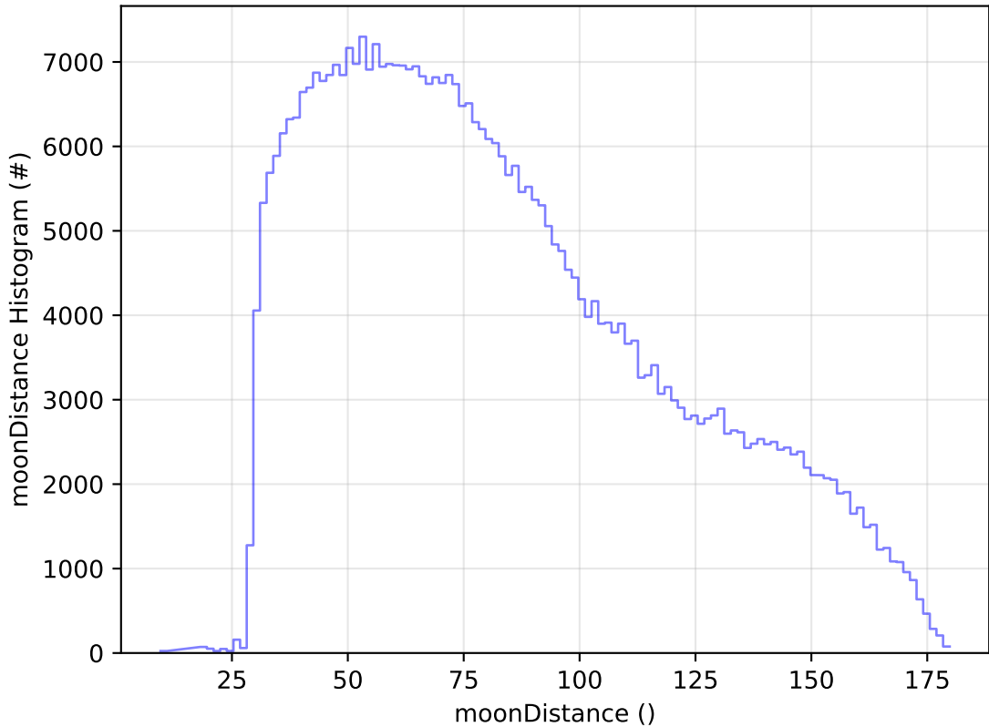
ddf_acor_sf10_lsf40_lsr20_v3.4_10yrs All sky z band: moonDistance Histogram
