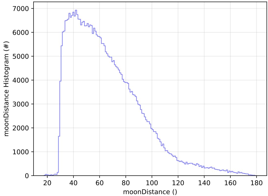
ddf_acor_sf10_lsf40_lsr20_v3.4_10yrs All sky y band: moonDistance Histogram
