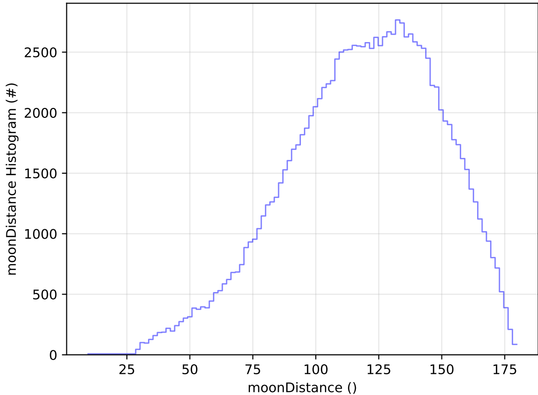
ddf_acor_sf10_lsf40_lsr20_v3.4_10yrs All sky u band: moonDistance Histogram
