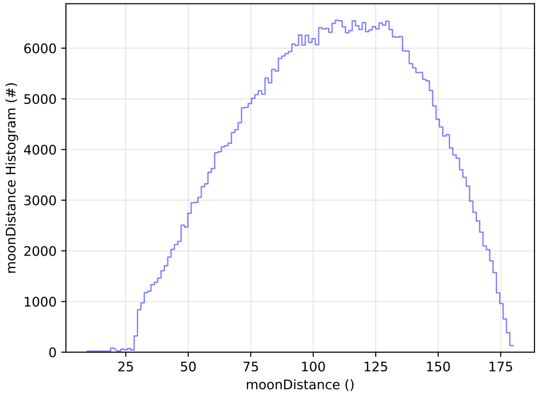
ddf_acor_sf10_lsf40_lsr20_v3.4_10yrs All sky r band: moonDistance Histogram
