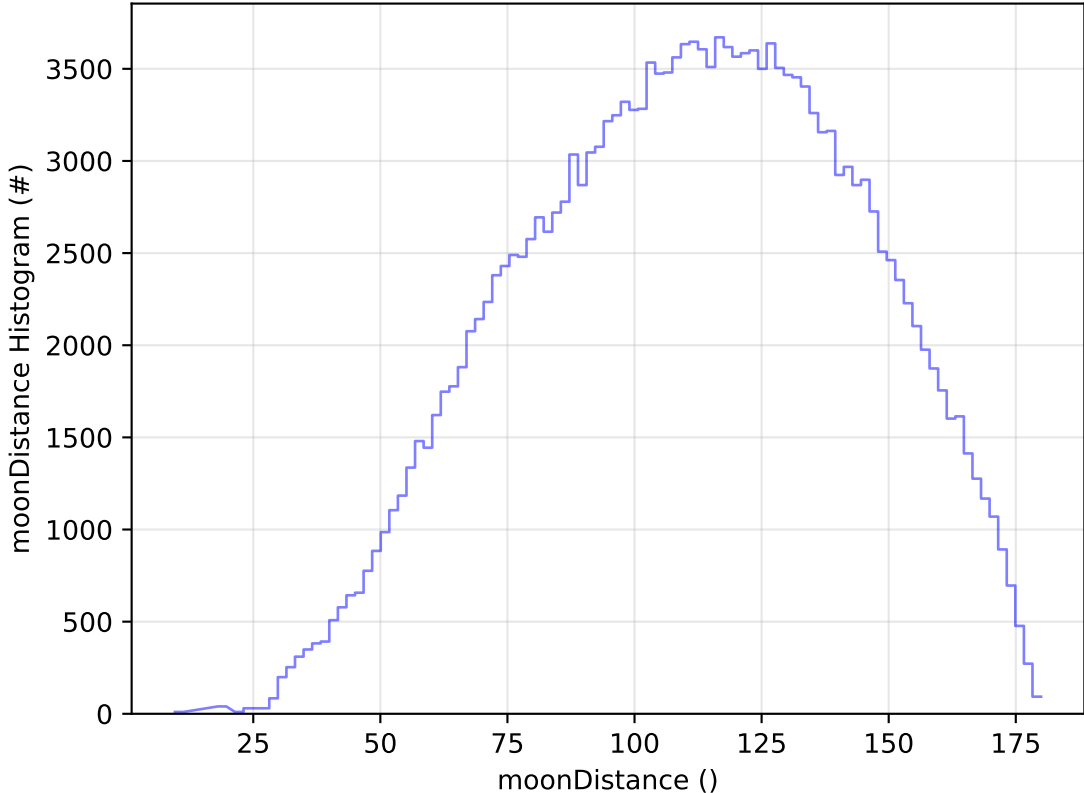
ddf_acor_sf10_lsf40_lsr20_v3.4_10yrs All sky g band: moonDistance Histogram
