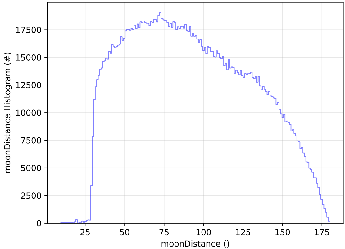
ddf_acor_sf10_lsf40_lsr20_v3.4_10yrs All sky all bands: moonDistance Histogram
