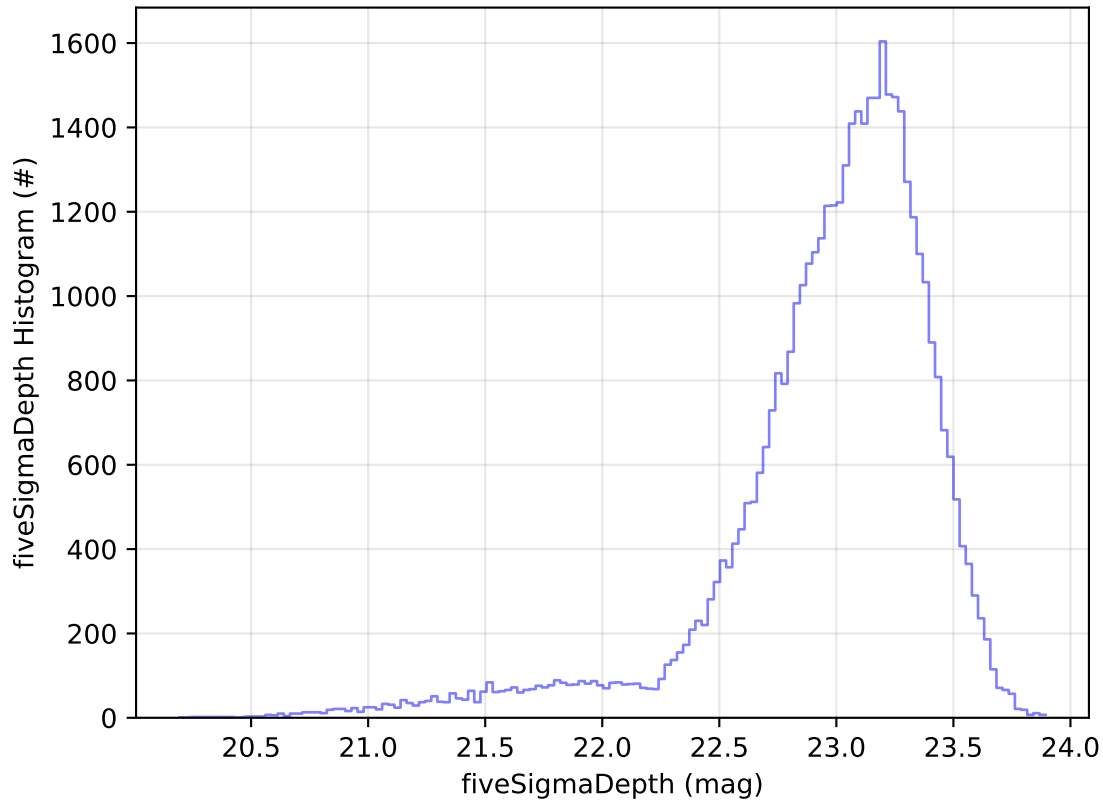
ddf_acor_sf10_lsf40_lsr20_v3.4_10yrs Yr 1 z band: fiveSigmaDepth Histogram
