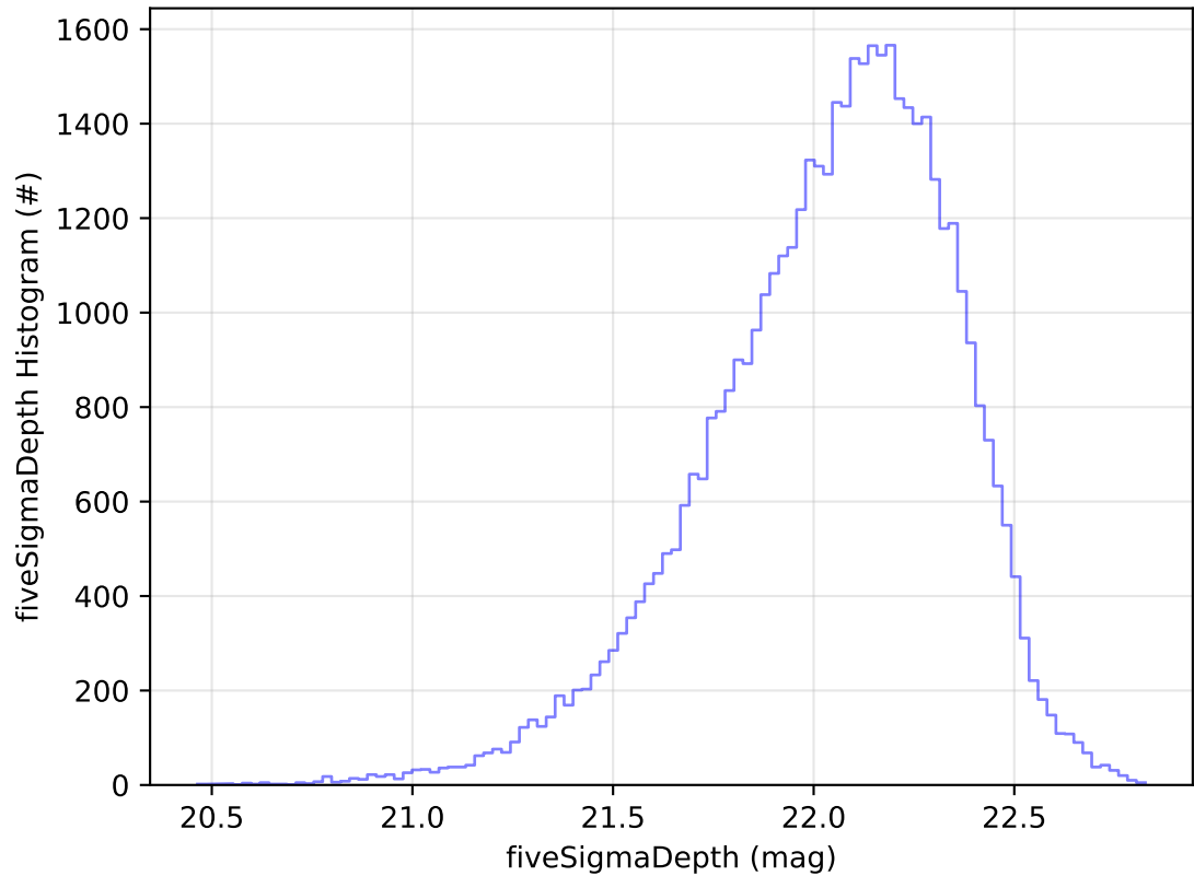
ddf_acor_sf10_lsf40_lsr20_v3.4_10yrs Yr 1 y band: fiveSigmaDepth Histogram
