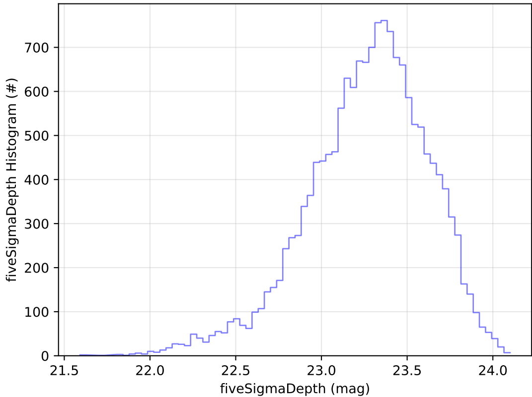
ddf_acor_sf10_lsf40_lsr20_v3.4_10yrs Yr 1 u band: fiveSigmaDepth Histogram
