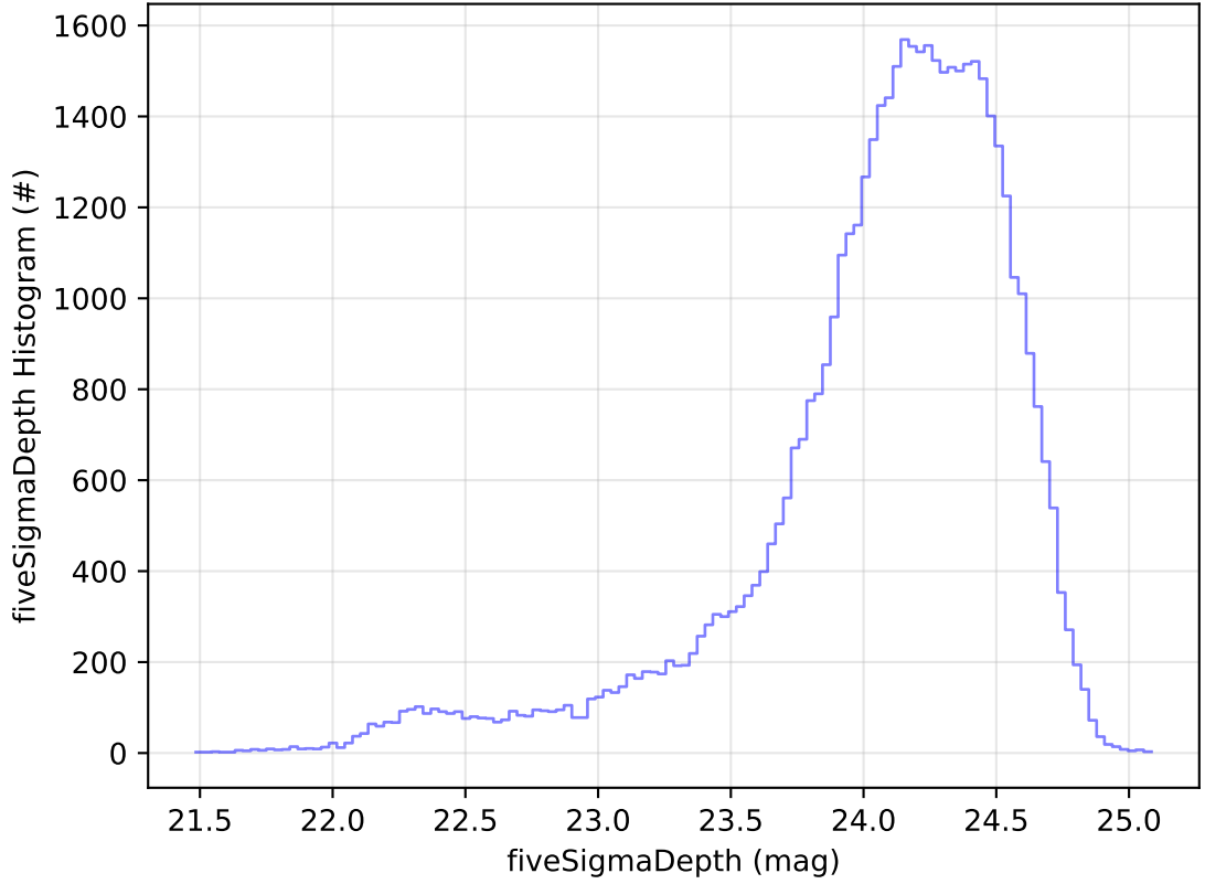
ddf_acor_sf10_ls40_lsr20_v3.4_10yrs Yr 1 r band: fiveSigmaDepth Histogram
