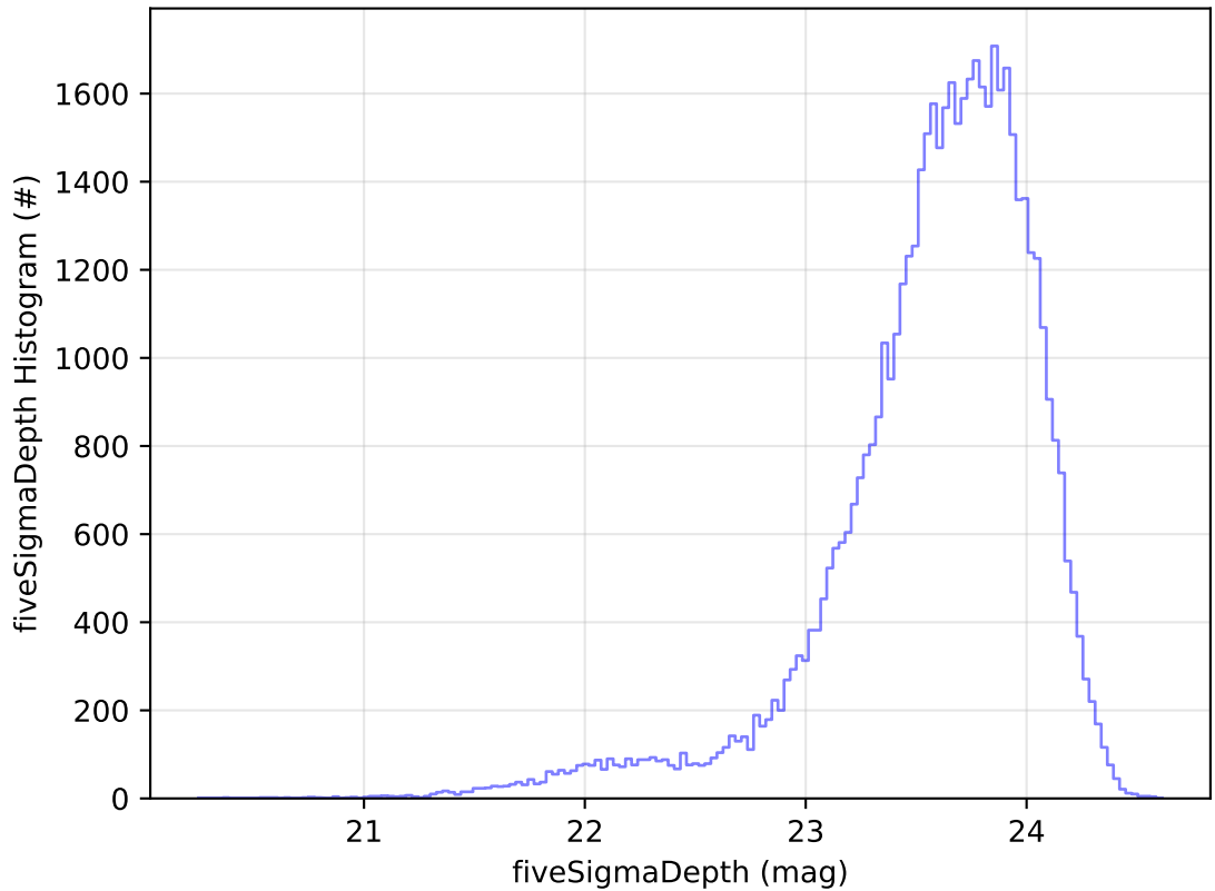
ddf_acor_sf10_lsf40_lsr20_v3.4_10yrs Yr 1 i band: fiveSigmaDepth Histogram
