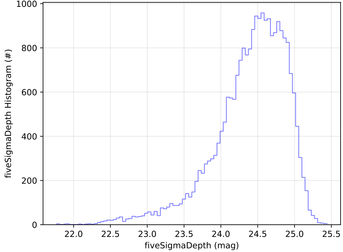
ddf_acor_sf10_lsf40_lsr20_v3.4_10yrs Yr 1 g band: fiveSigmaDepth Histogram
