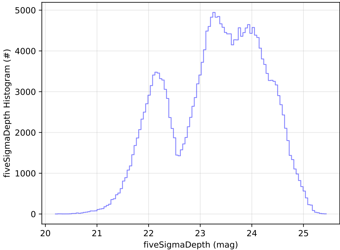
ddf_acor_sf10_lsf40_lsr20_v3.4_10yrs Yr 1 all bands: fiveSigmaDepth Histogram
