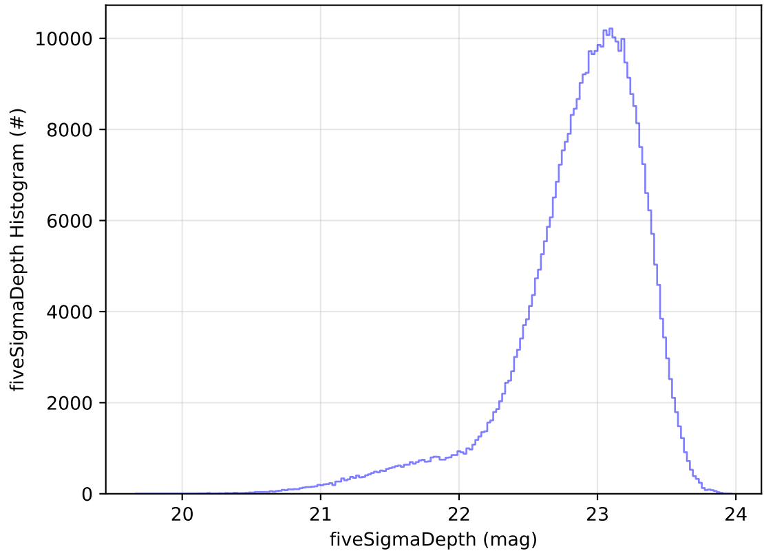
ddf_acor_sf10_lsf40_lsr20_v3.4_10yrs WFD z band: fiveSigmaDepth Histogram
