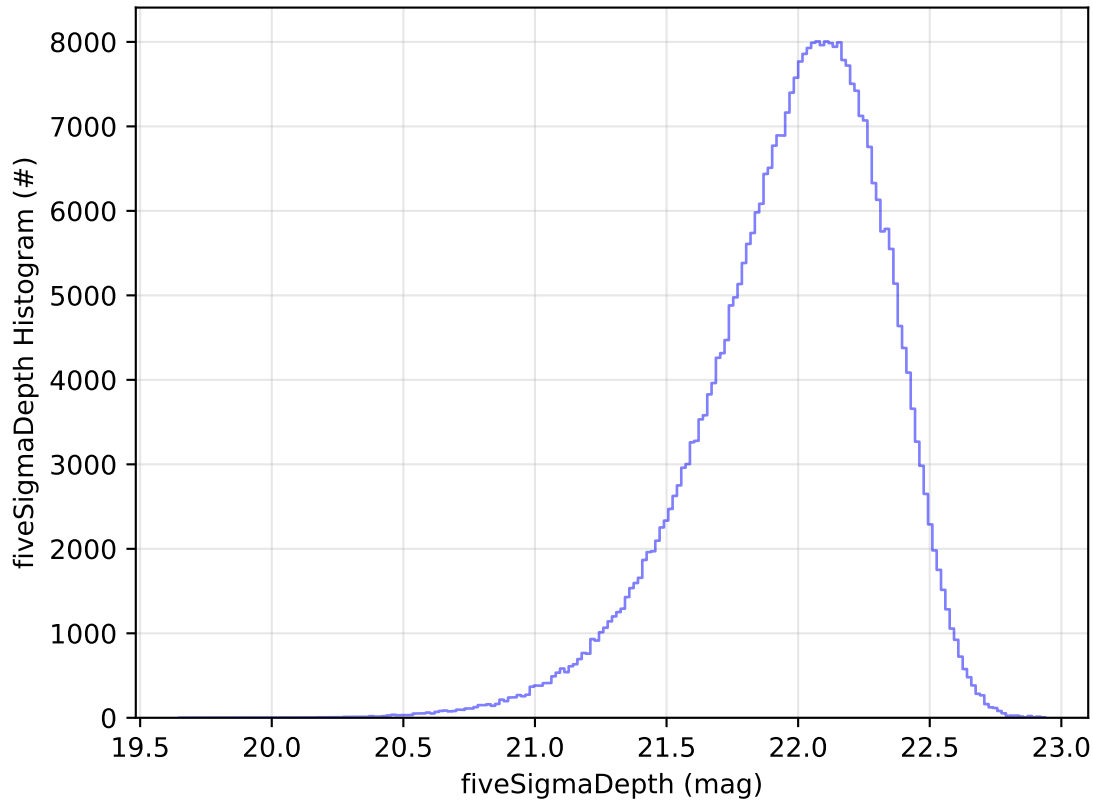
ddf_acor_sf10_lsf40_lsr20_v3.4_10yrs WFD y band: fiveSigmaDepth Histogram
