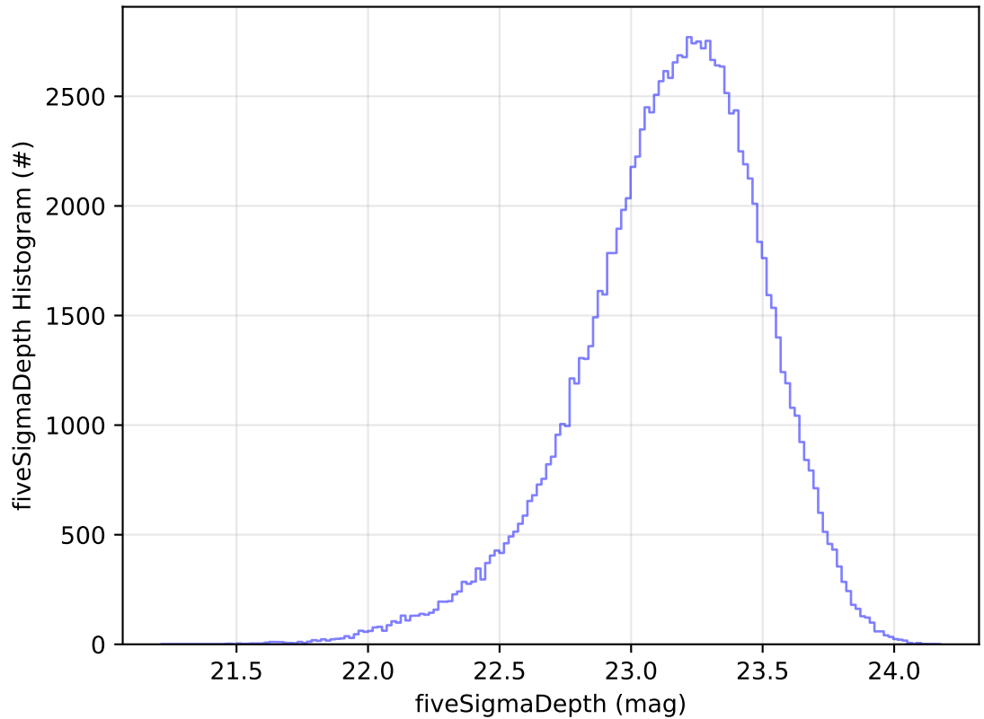
ddf_acor_sf10_lsf40_lsr20_v3.4_10yrs WFD u band: fiveSigmaDepth Histogram
