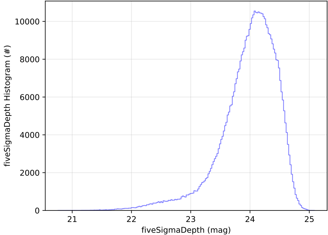
ddf_acor_sf10_lsf40_lsr20_v3.4_10yrs WFD r band: fiveSigmaDepth Histogram
