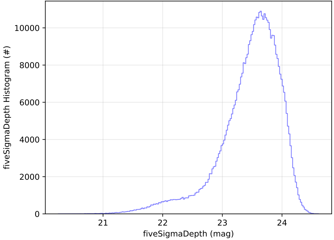
ddf_acor_sf10_lsf40_lsr20_v3.4_10yrs WFD i band: fiveSigmaDepth Histogram
