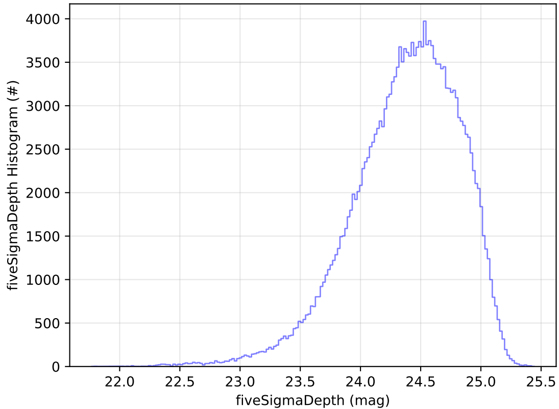
ddf_acor_sf10_lsf40_lsr20_v3.4_10yrs WFD g band: fiveSigmaDepth Histogram
