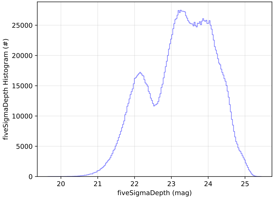
ddf_acor_sf10_lsf40_lsr20_v3.4_10yrs WFD all bands: fiveSigmaDepth Histogram
