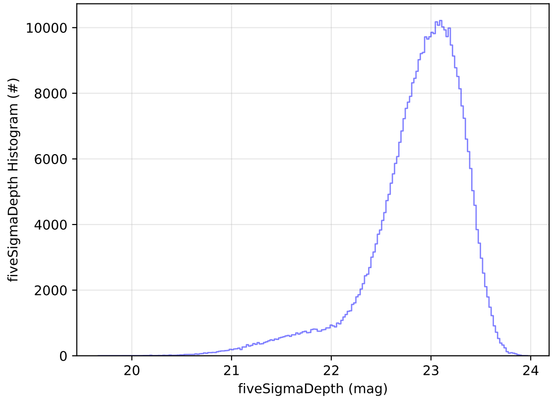
ddf_acor_sf10_lsf40_lsr20_v3.4_10yrs All sky z band: fiveSigmaDepth Histogram
