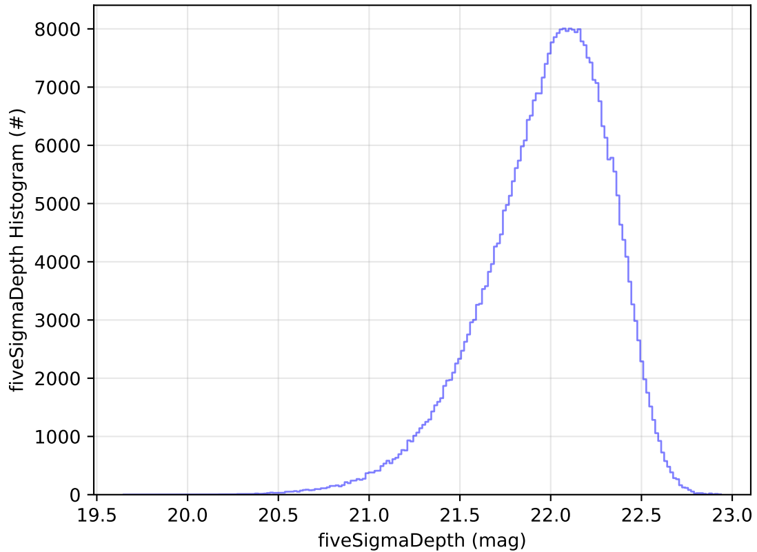
ddf_acor_sf10_lsf40_lsr20_v3.4_10yrs All sky y band: fiveSigmaDepth Histogram
