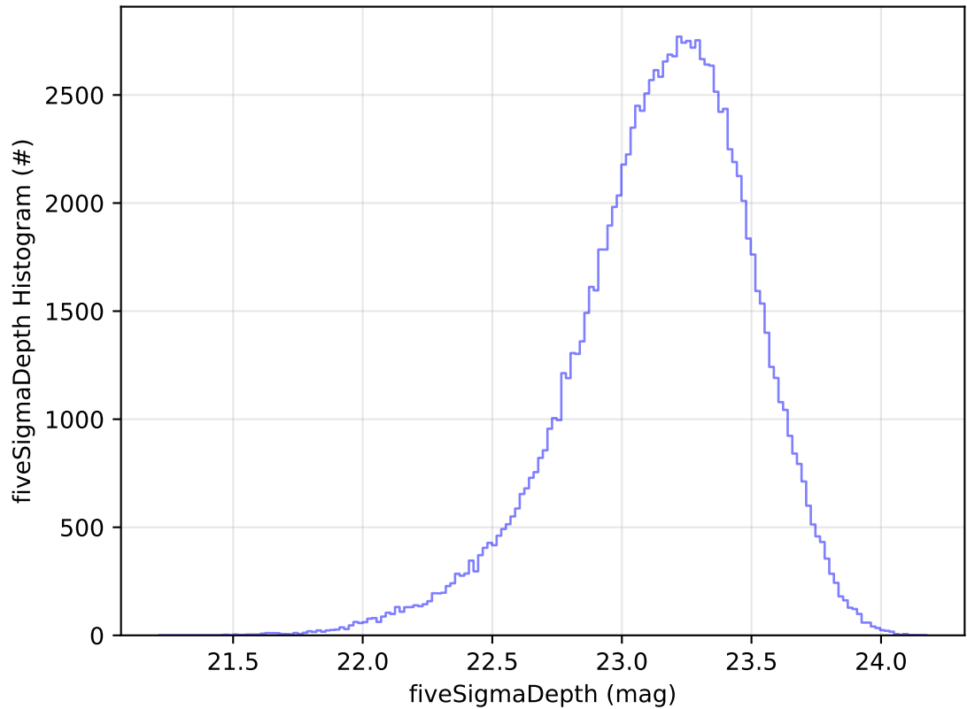
ddf_acor_sf10_lsf40_lsr20_v3.4_10yrs All sky u band: fiveSigmaDepth Histogram
