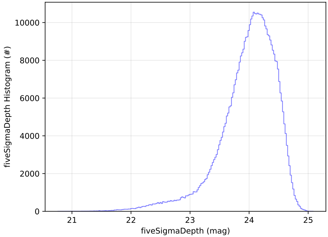
ddf_acor_sf10_lsf40_lsr20_v3.4_10yrs All sky r band: fiveSigmaDepth Histogram
