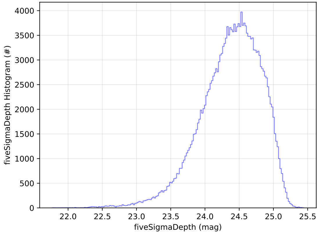
ddf_acor_sf10_lsf40_lsr20_v3.4_10yrs All sky g band: fiveSigmaDepth Histogram
