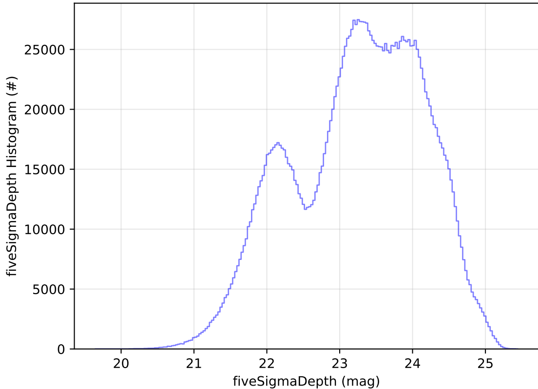
ddf_acor_sf10_lsf40_lsr20_v3.4_10yrs All sky all bands: fiveSigmaDepth Histogram
