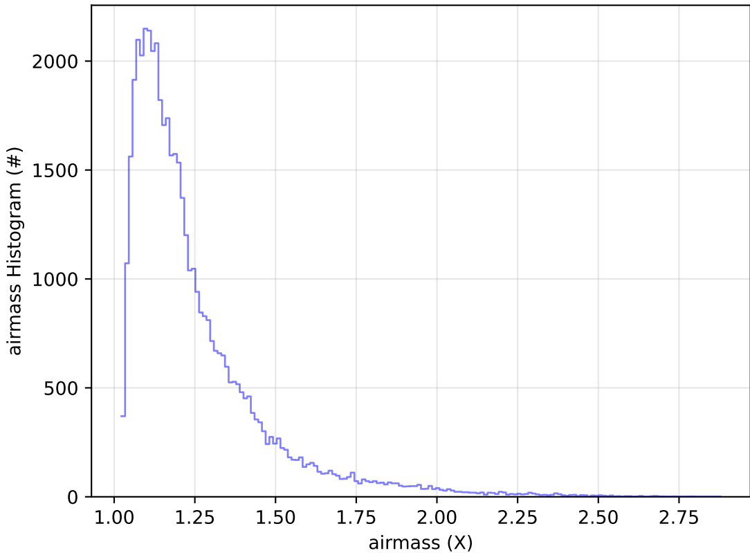
ddf_acor_sf10_ls40_lsr20_v3.4_10yrs Yr 1 y band: airmass Histogram
