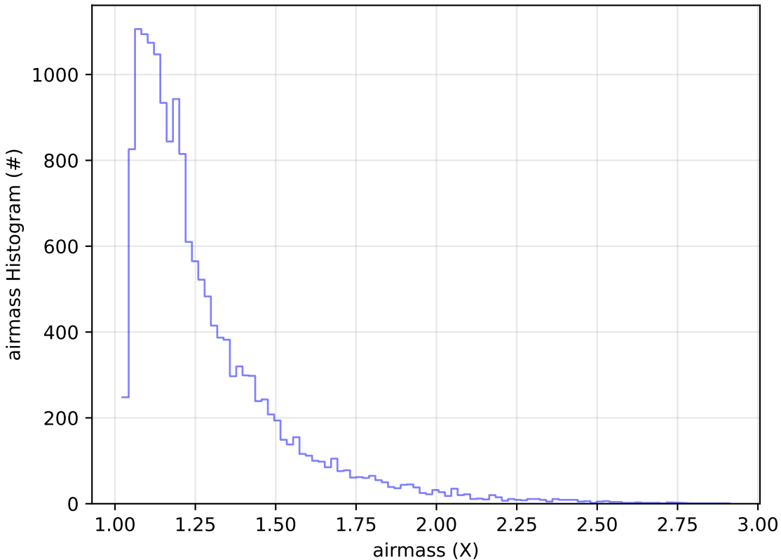
ddf_acor_sf10_lsf40_lsr20_v3.4_10yrs Yr 1 u band: airmass Histogram
