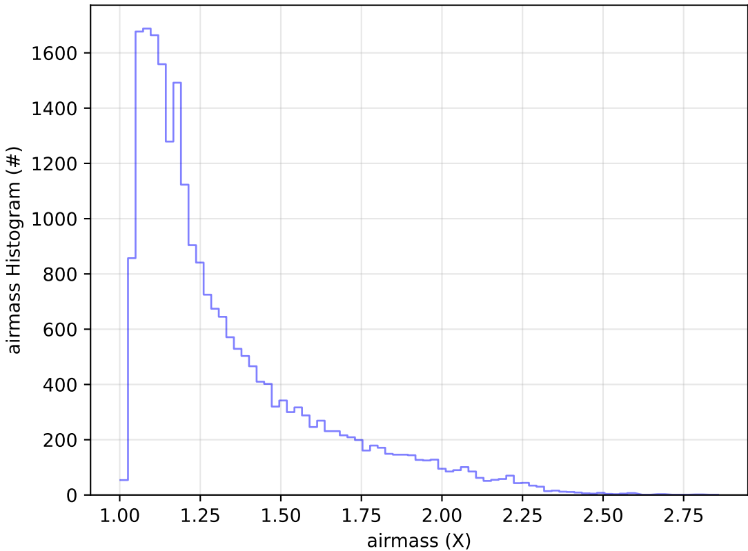
ddf_acor_sf10_lsf40_lsr20_v3.4_10yrs Yr 1 g band: airmass Histogram
