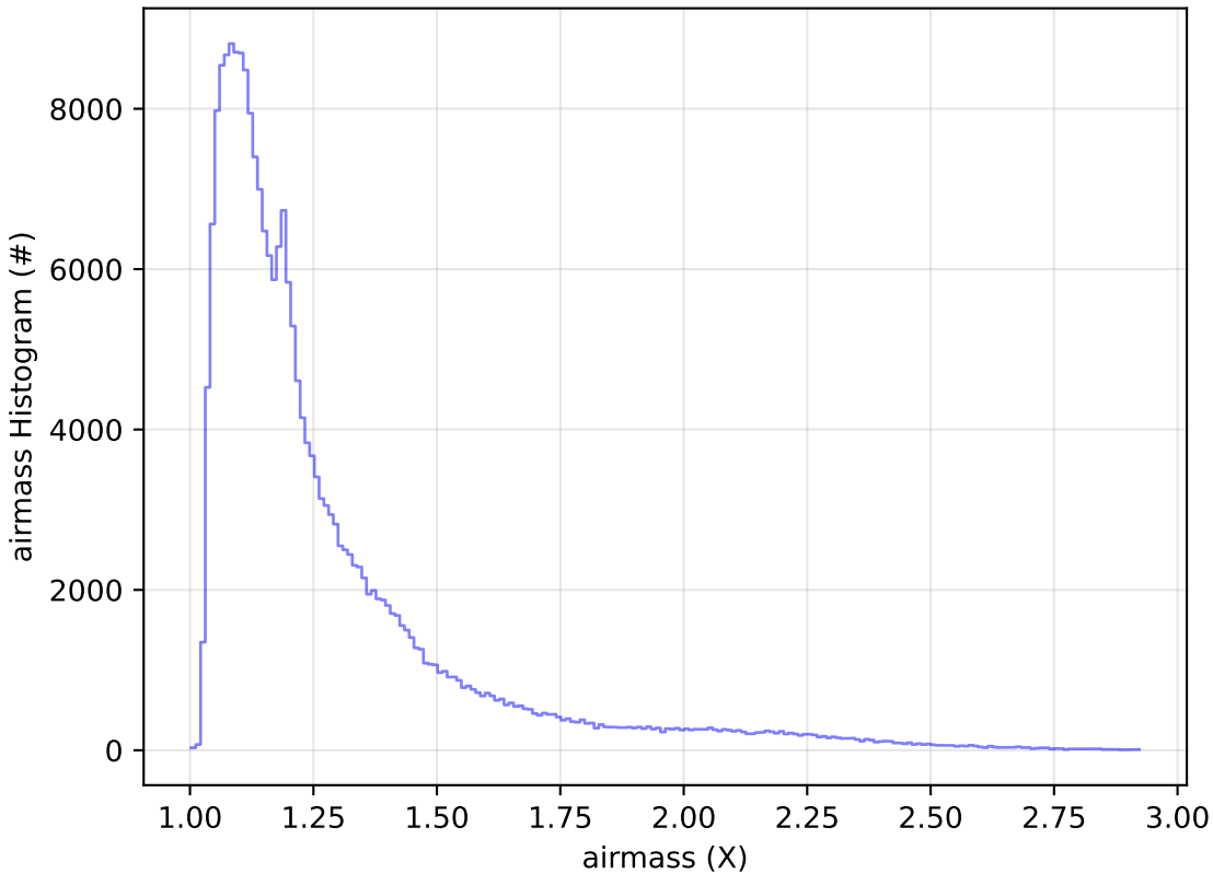
ddf_acor_sf10_lsf40_lsr20_v3.4_10yrs Yr 1 all bands: airmass Histogram
