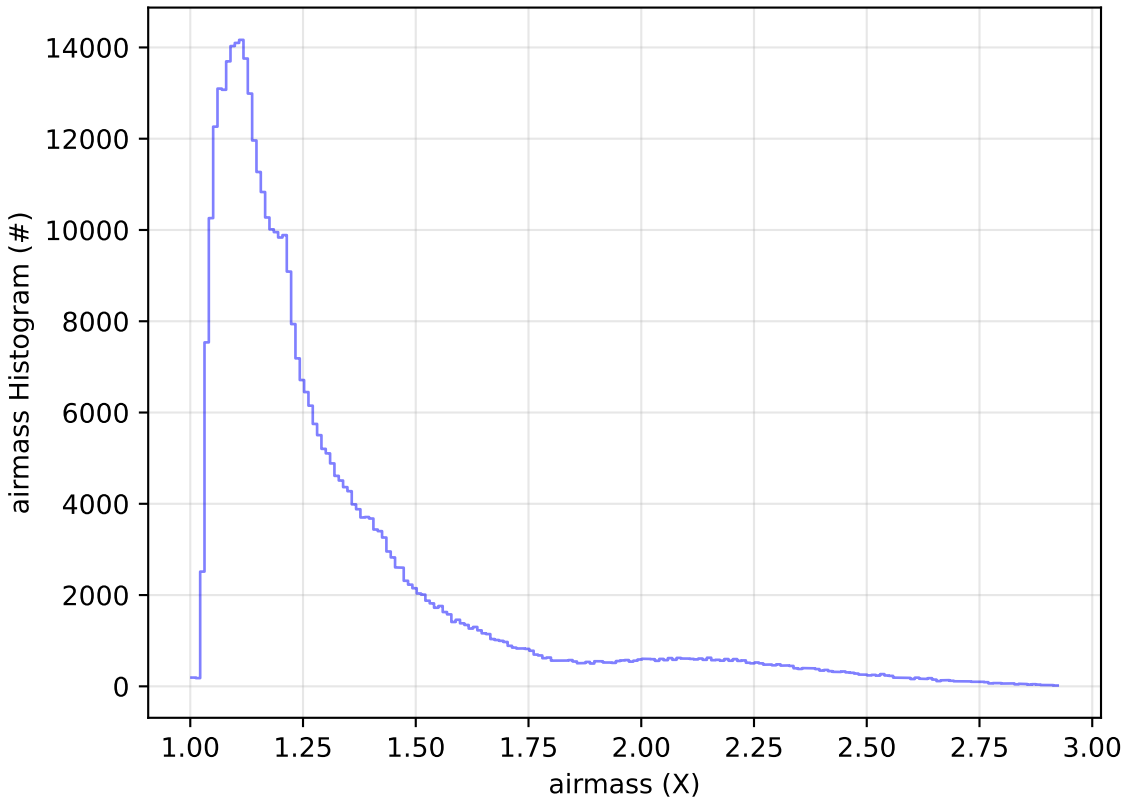
ddf_acor_sf10_lsf40_lsr20_v3.4_10yrs WFD z band: airmass Histogram
