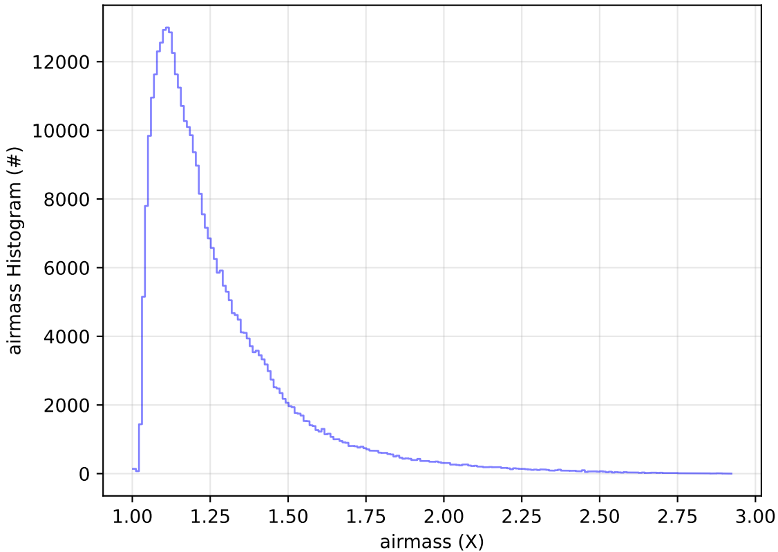
ddf_acor_sf10_lsf40_lsr20_v3.4_10yrs WFD y band: airmass Histogram
