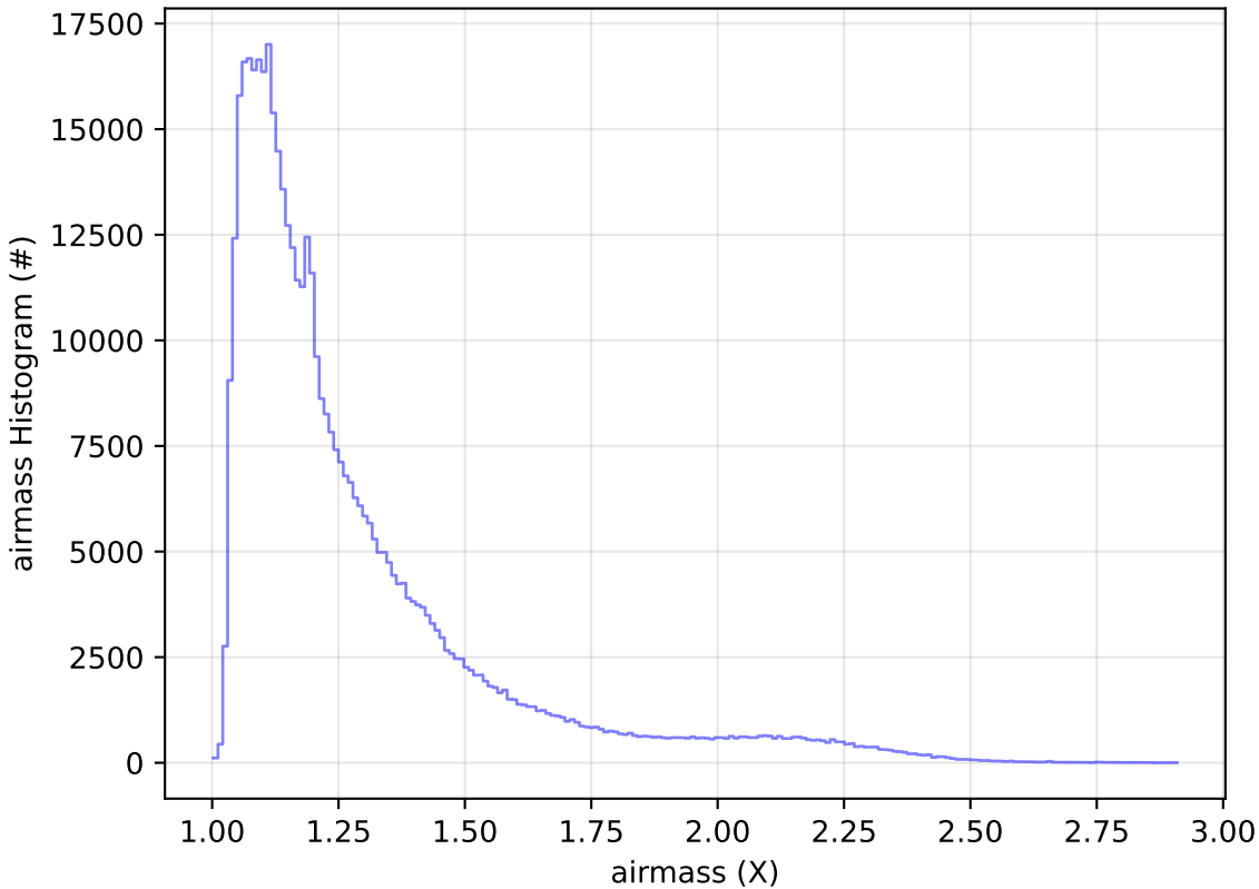
ddf_acor_sf10_lsf40_lsr20_v3.4_10yrs WFD r band: airmass Histogram
