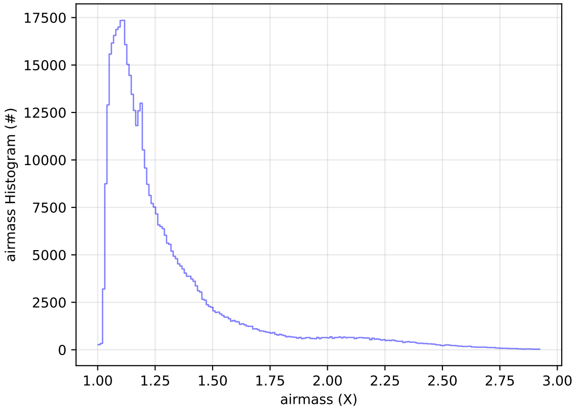
ddf_acor_sf10_lsf40_lsr20_v3.4_10yrs WFD i band: airmass Histogram
