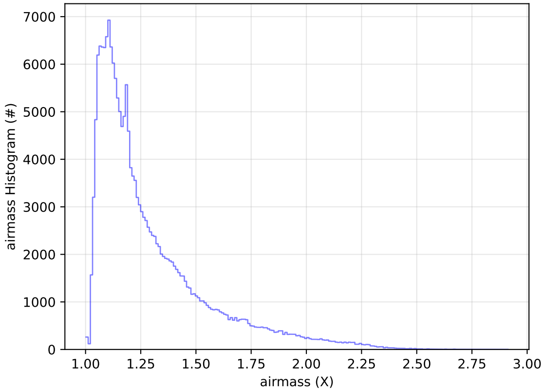
ddf_acor_sf10_lsf40_lsr20_v3.4_10yrs WFD g band: airmass Histogram
