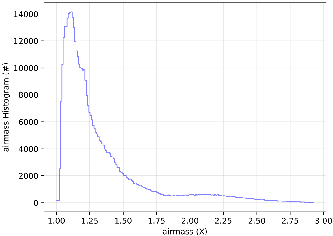
ddf_acor_sf10_lsf40_lsr20_v3.4_10yrs All sky z band: airmass Histogram
